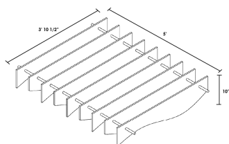
Overall Dimensions
